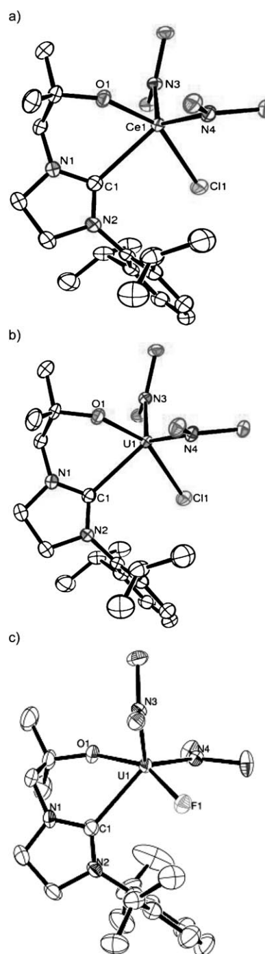
Figure 1. Displacement ellipsoid drawings of the molecular structures of a) [Ce(L)(N'') 2 Cl], b) [U(L)(N'') 2 Cl], and c) [U(L)(N'') 2 F]. Lattice solvent molecules, hydrogen atoms and silyl methyl groups are omitted for clarity.
